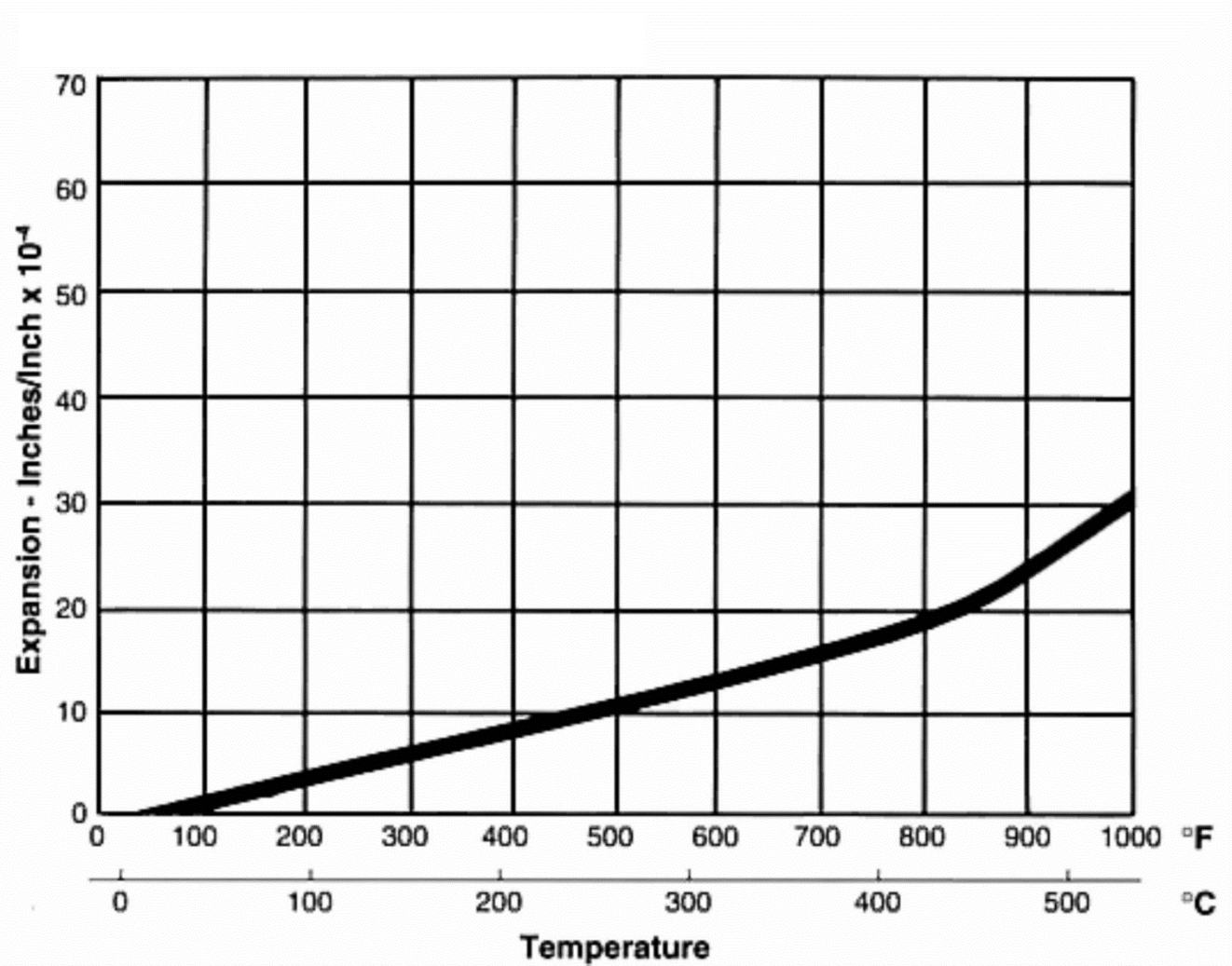
Thermal Expansion Curve
